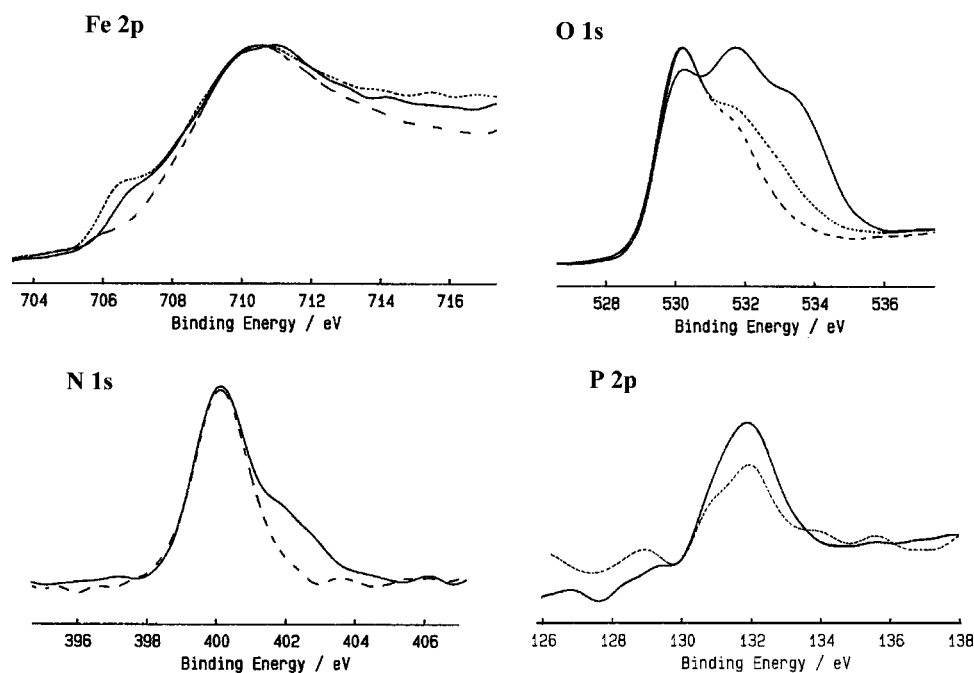
Fig. 6. Comparison of the XPS spectra of Fe 2p, O 1s, N 1s, P 2p regions obtained for carbon steel surface after 2 h of immersion in the solutions containing (---) 50 mg l -1 FA; (- - -) 200 mg l -1 PCAS; (—) 200 mg l -1 PCAS + 50 mg l -1 FA.
